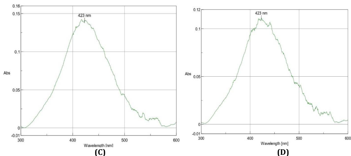
Fig 4: UV spectra of Eltrombopag Olamine (10 µg/ml) obtained in the stress degradation assays using Acidic (A), Basic (B), Oxidative(C), Photolytic (D)
