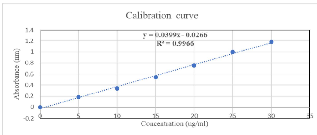
Fig 3: Calibration curve plot of Eltrombopag Olamine at 423nm
