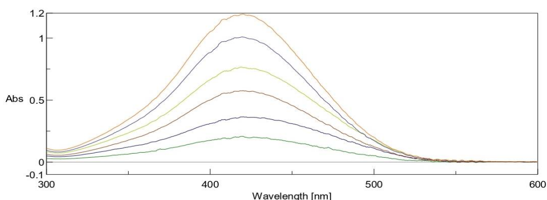
Fig 4: Overly spectrum of Eltrombopag Olamine (5 to 30 \mu\text{g/ml} ) at 423 nm
