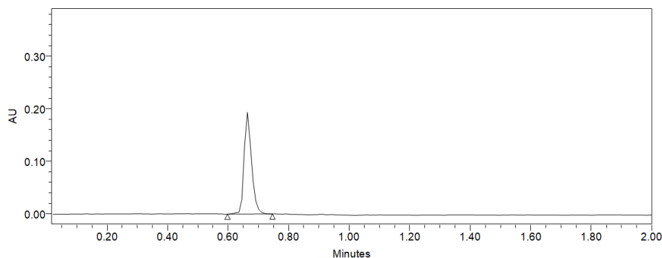
Fig. 2: Optimized chromatogram of BLMX
