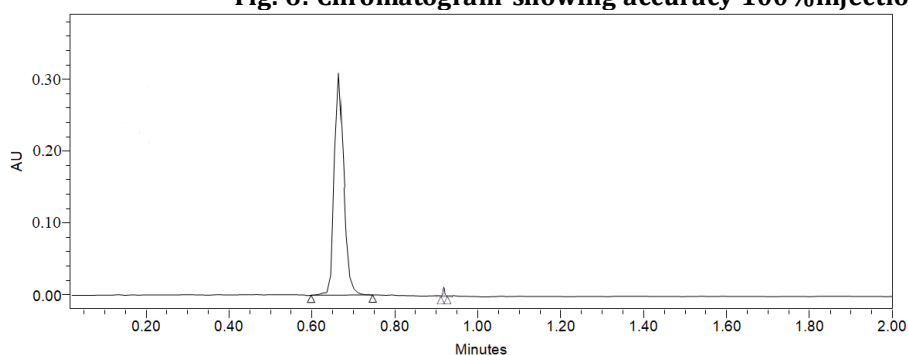
Fig. 7: Chromatogram showing accuracy 150%injection
