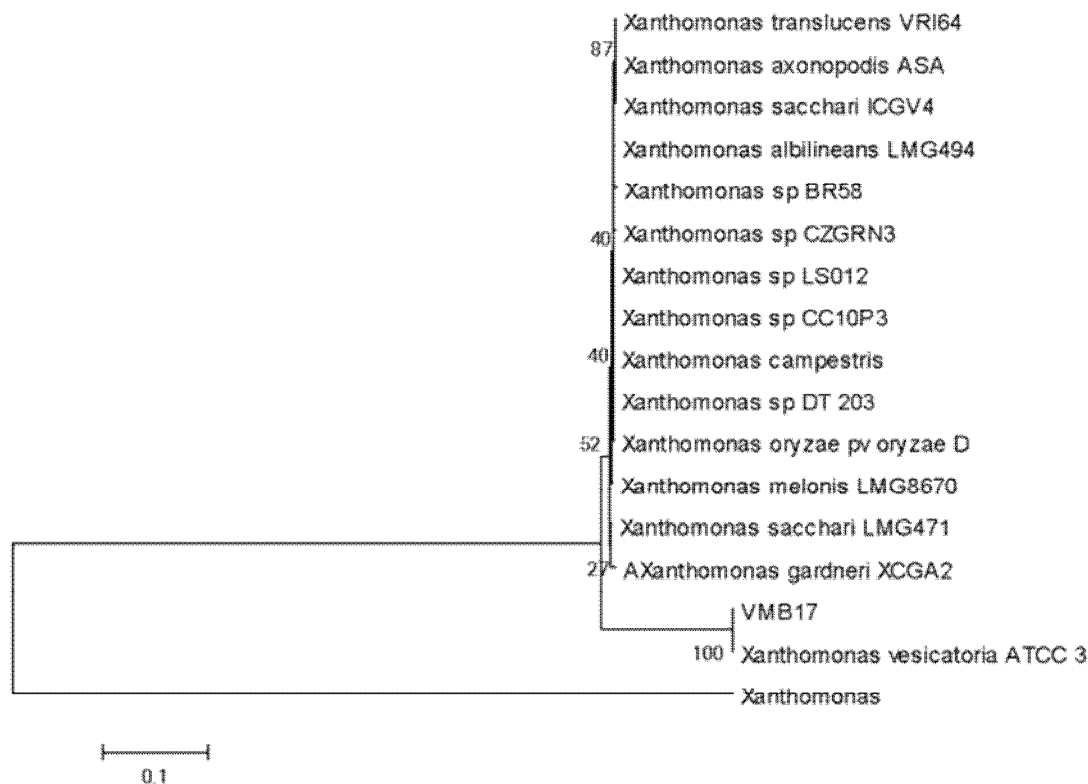
FIGURE 1: PHYLOGENETIC PLACEMENT OF VMB17 (DDBJ ACCESSION NUMBER LC530855) BASED ON 16S rRNA ANALYSIS
