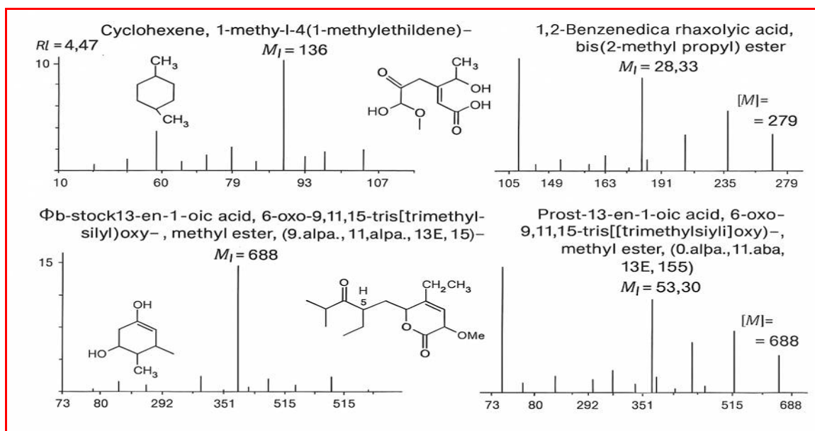
Fig. 2: Representative Mass Spectra of Selected Compounds from Euphorbia milii Flower Extract
