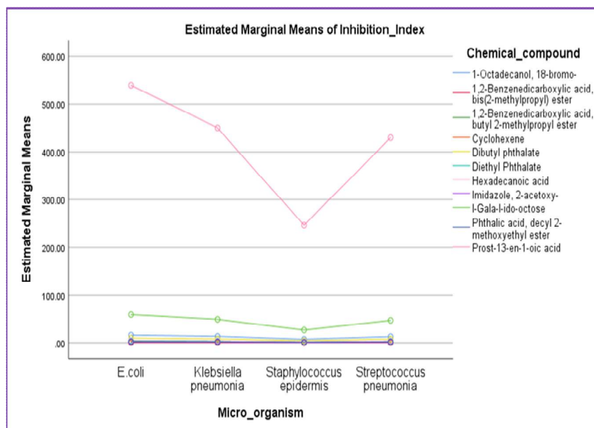
Fig.7: Inhibition indices of chemical compounds against the four microorganisms for flower extract
