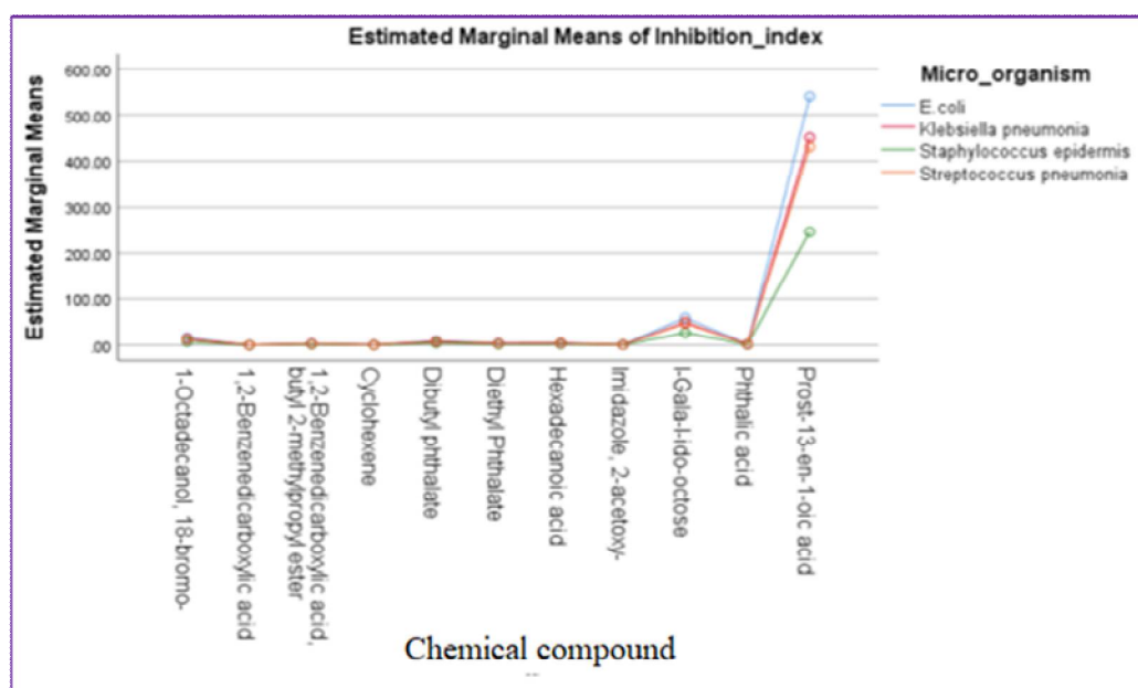
Fig.6: Interaction between chemical compounds and microorganisms on the inhibition index for flower extract
