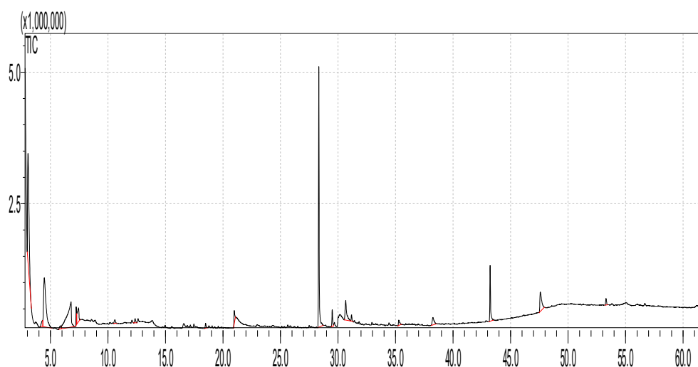
Fig. 1: GC-MS chromatogram of Euphorbia milii flower sample
