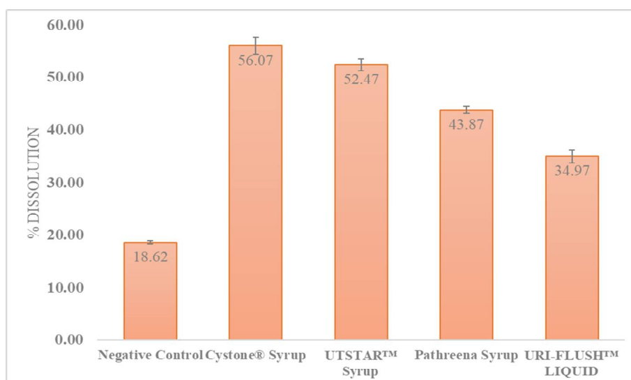
Fig. 1: CaOx Dissolution activity of negative control and Commercial samples
