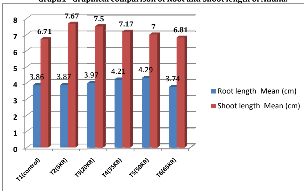
Graph1 -Graphical comparison of Root and Shoot length of Alfalfa.
