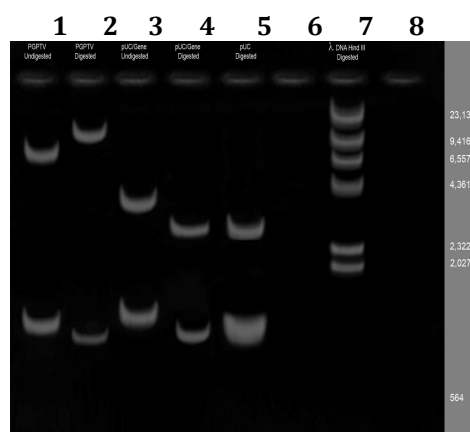
Fig 2. Comparison of digested and undigested plasmids. Lane 1 – pGPTV undigested, Lane 2 – pGPTV digested with XbaI and EcoRI , Lane 3 – pUC18/ Bt-cry1Ac gene undigested, Lane 4 – pUC18/ Bt-cry1Ac gene digested with XbaI and EcoRI , Lane 5 – pUC18 digested. Lane 6, 8 – empty, Lane 7 \lambda DNA with HindIII digest.
