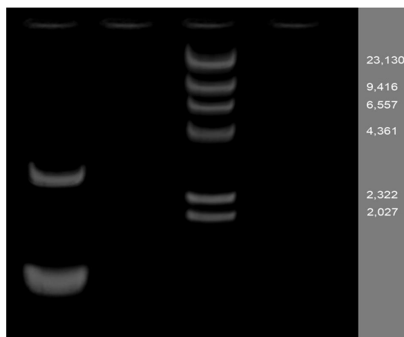
Fig 8. Detection of Transgenes. Plasmid DNA was isolated and analysed by PCR using the forward primer 5'CTGAATGAACTGCAGGACGAGG3' and reverse primer 5'GCC AACGCTATGTCCTGATAGC 3'. Amplified products were fractionated by agarose gel electrophoresis. Lane 1, Transformed A. tumefaciens formed band of 2.6 kb size, Lane 2, Non transformants does not produce bands, Lane 3, \lambda DNA.
