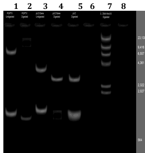
Fig 3. Gel elution. Lane 1 – pGPTV undigested, Lane 2 – pGPTV digested with XbaI and EcoRI , Lane 3 – pUC18/ Bt-cry1Ac gene undigested, Lane 4 – pUC18/ Bt-cry1Ac gene digested with XbaI and EcoRI , Lane – 5 pUC18 digested. Lane 6, 8 – empty, Lane 7 – \lambda DNA with HindIII digest. pGPTV vector from Lane – 213 kb and Bt-cry1Ac gene released from pUC18 showing 1363 bp are eluted from the gel for further process.
