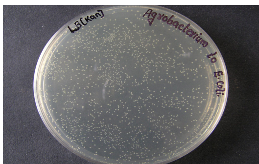
Fig 8. Back transformation transferring the gene from A. tumefaciens to E.coli , to check the presence of the gene.
