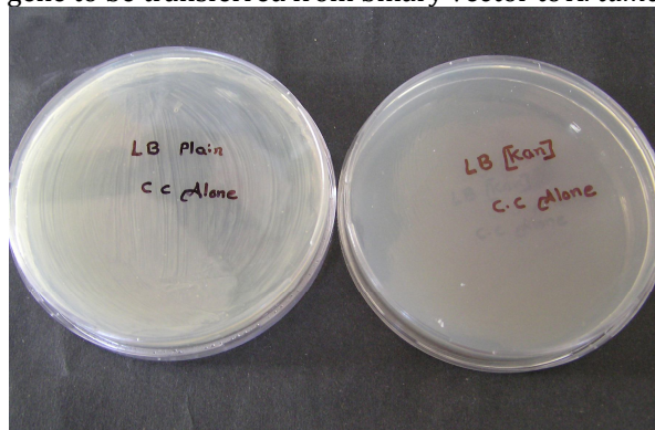
Fig 4. Competence Cells (CC) after transformation spreaded on plain LB plain plate (Plate – 1) and on LB with Kanamycin plate (Plate – 2)
