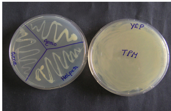
Fig 6. Triparental mating plates, from left to right (plate - 1) master plate , (plate - 2) triparental mating (TPM) plate, mixture of A. tumefaciens (LBA 4404) strain, helper strain (pRK2013) and binary vector with desired gene (pGPTV+ Bt-cry1Ac )
