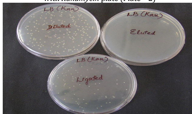
Fig 5. Transformation plates Competence Cell with diluted plasmid (Plate – 3) on Kanamycin plate, eluted sample on Kanamycin plate (pGPTV, Plate – 4), ligated sample (pGPTV + Bt-cry1Ac gene, Plate - 5)
