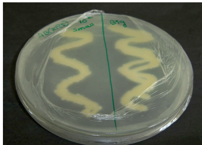
Fig 7. AB (KRS) Plate 10^{-3} dilution after colonization streaked on a new AB (KRS) plate and can be used for co - cultivation
