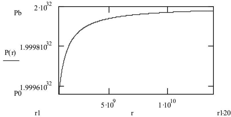
Fig.2. Radial distribution of ether pressure for the Sun.
