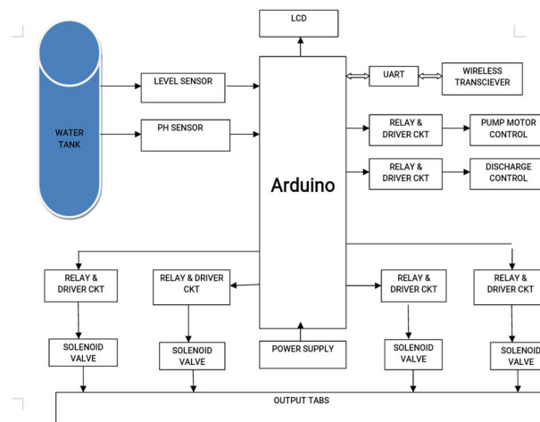
FIGURE 2 -BLOCK DIAGRAM
